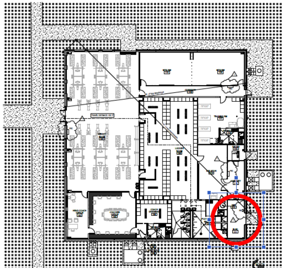
1 LIFE SAFETY PLAN LS101
